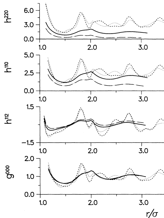
FIG. 2. Projections of the pair distribution function of dipolar hard spheres at \mu^*=2.5 . Solid line: \rho^*=0.9 , \epsilon'=\infty (fluid); contact values are g^{000}=8.4 , h^{112}=10.3 , h^{110}=19.0 , and h^{220}=18.5 . Dotted line: \rho^*=1.01 , \epsilon'=\infty (bco); contact values are g^{000}=7.2 , h^{112}=9.7 , h^{110}=18.7 , and h^{220}=23.7 . Dashed line: \rho^*=1.005 , \epsilon'=\infty (bct); contact values are g^{000}=7.5 , h^{112}=9.6 , h^{110}=19.6 , and h^{220}=25.1 . Dot-dashed line: \rho^*=0.916 , \epsilon'=1 (fluid); contact values are g^{000}=8.8 , h^{112}=10.8 , h^{110}=17.4 , and h^{220}=14.8 .
